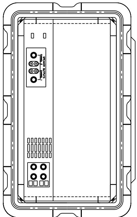
REAR VIEW (WITH LIDS REMOVED)
