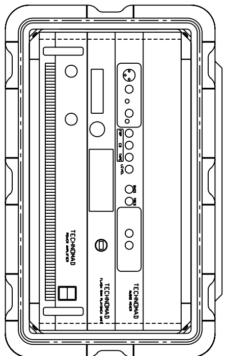
FRONT VIEW (WITH LIDS REMOVED)
